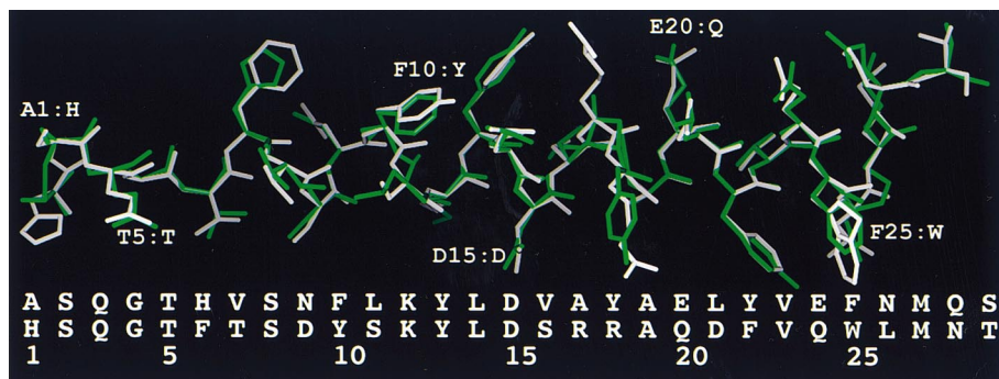
Figure 3 Superposition of 1gc and model built by TEXTAL . This figure and all color figures were produced using the program SPOCK (Christopher, 1998). The sequence on top is for the model built by TEXTAL , as is the structure in green.
