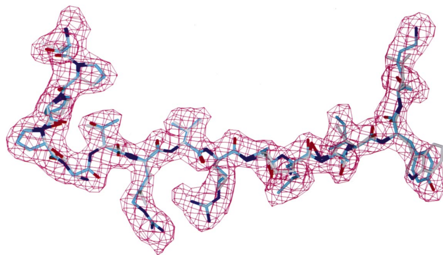
Figure 4 Region in 1tup compared with the model built by TEXTAL . Shown are residues 147–155. The figure includes a 1 \sigma contour of the electron-density map of 1tup. In this and in Fig. 5, the TEXTAL model C atoms are in white and the C atoms of the original PDB structure (here, 1tup.pdb) are in light blue; all N atoms for both are dark blue, all O atoms are red and all S atoms are yellow.
